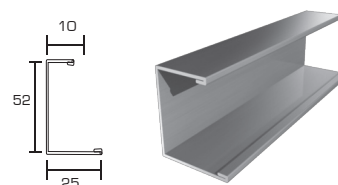
PROFILO A "C" 25X52X10 L=4000 mm
