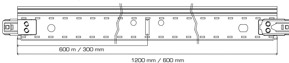
Cross T (Vinkel T-profil) 1200 mm / 600 mm
